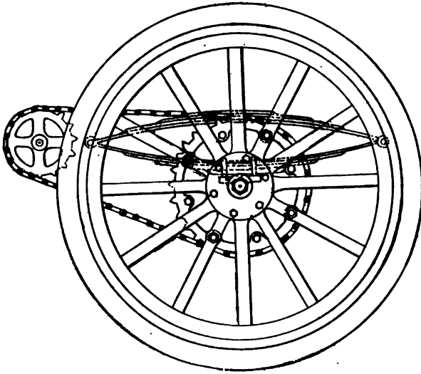
FIG. 84.—Wooden Wheel, such as is used on heavy gasoline carriages of Panhard, Mera and others. It turns loose on the axle and is driven by a sprocket on a counter-shaft.
